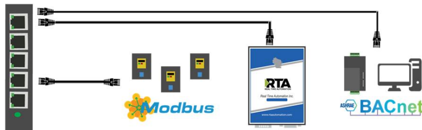
TCP/IP Servers 460MCBC-N34 IP Servers
